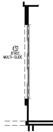
KITCHEN 9', 12', or 15' SLIDER OPTION
